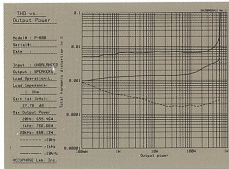
• OUTPUT POWER vs. TOTAL HARMONIC DISTORTION (at 1 ohms, LOW IMP mode)
