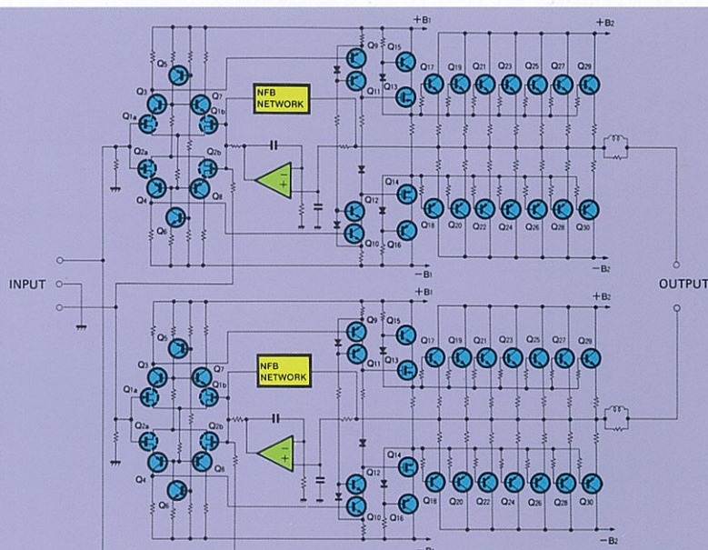
Fig. 2 Block Diagram of P-800 (One-Channel)
