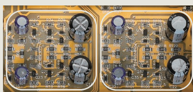
2-parallel circuit layout of MCS+ principle
