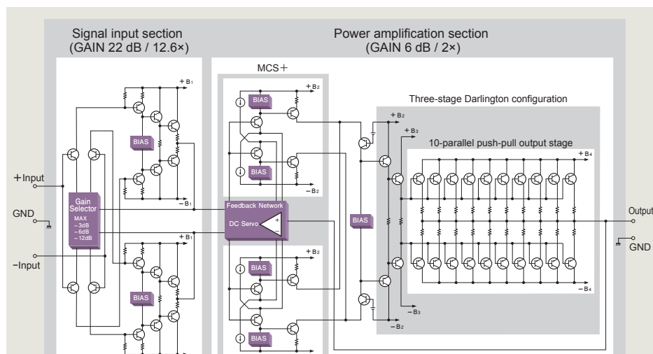
MCS+ circuitry
