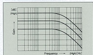
Fig. 4 Frequency response with current feedback (response remains uniform also when gain changes)
