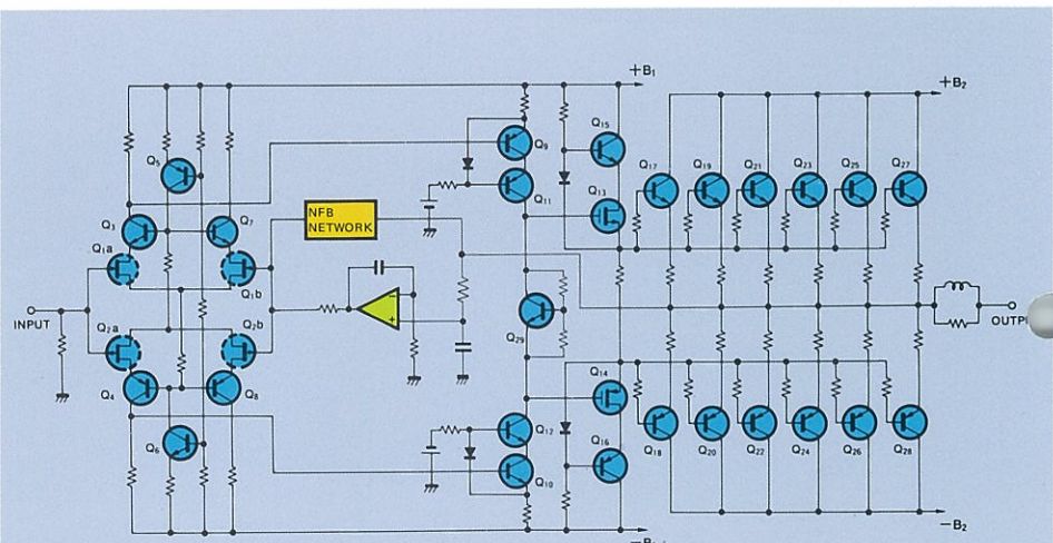
Fig. 1 P-500 Circuit Diagram
