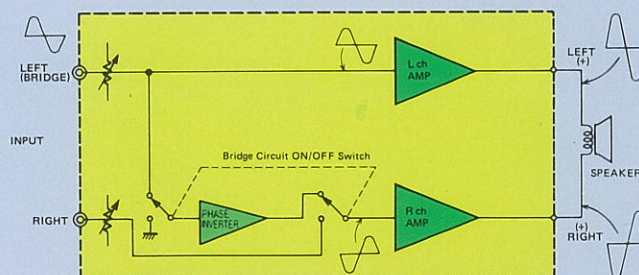
Fig. 2 Principle of the Bridge Connection
