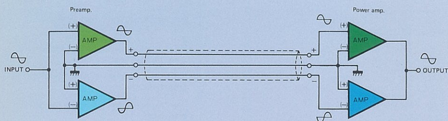
Fig. 3 Principle of the Balanced Type Network
