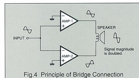
Fig. 4 Principle of Bridge Connection
