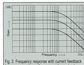
Fig. 3 Frequency response with current feedback (response remains uniform even when gain changes)
