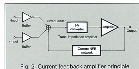
Fig. 2 Current feedback amplifier principle
