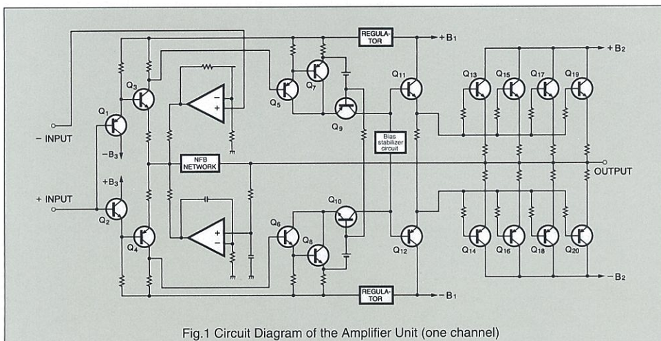
Fig. 1 Circuit Diagram of the Amplifier Unit (one channel)
