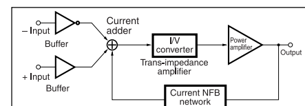
Figure 3 Principle of current feedback amplifier
