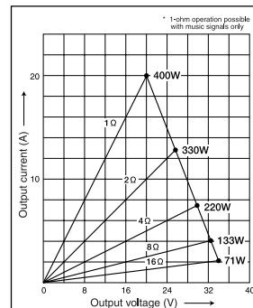
Figure 2 Load impedance vs. output power (output voltage/output current) of P-370
