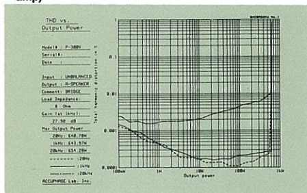
● OUTPUT POWER vs TOTAL HARMONIC DISTORTION CHARACTERISTIC (at 8 ohms load, as monophonic amp)
