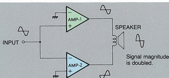
Fig. 2 Operating Principle of Bridge Connection
