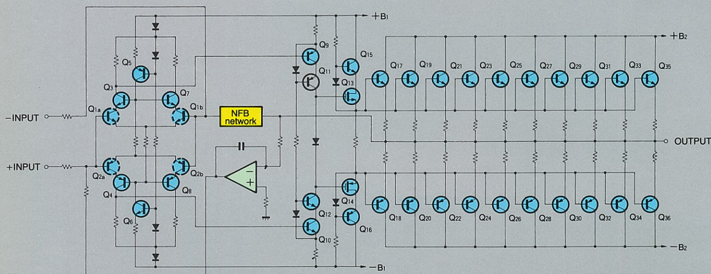
Fig. 1 P-300V Circuit Diagram
