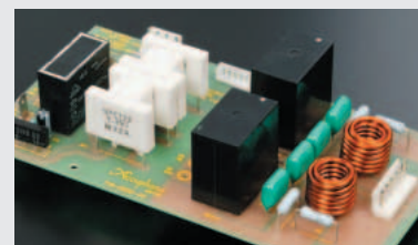
Output assembly
