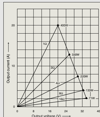
Fig. 2 Load impedance vs. output power (Output voltage/output current)
