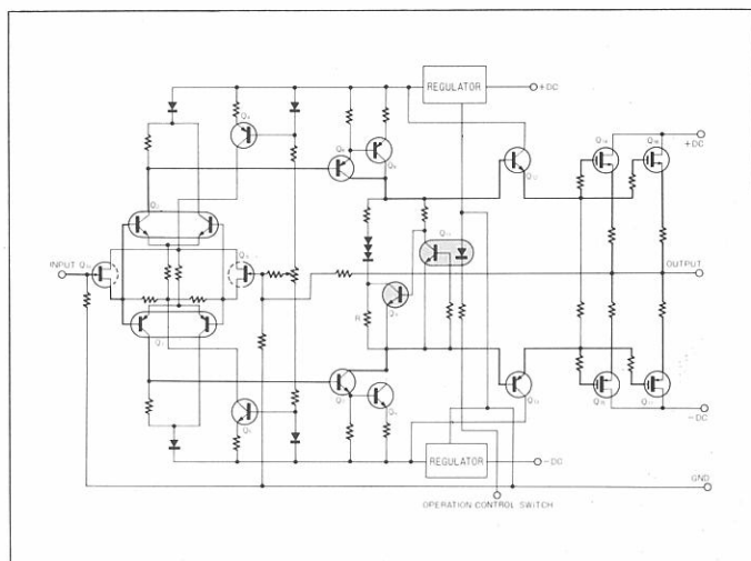
Fig.1 MOS FETs' SYMMETRICAL PUSH-PULL DC POWER AMPLIFIER
