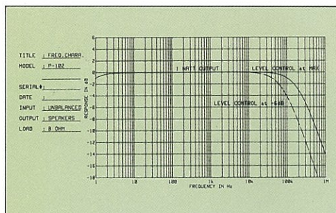
• Frequency response
