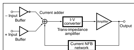
Fig. 3 Current feedback amplifier principle diagram
