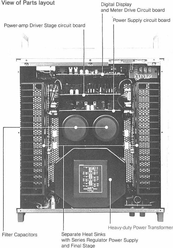
Top View of Parts layout
