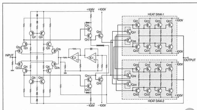
Fig. 1 Diagram of M-100's Amplifier Circuitry
