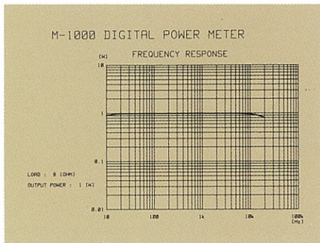
● FREQUENCY CHARACTERISTIC OF DIGITAL POWER METER
