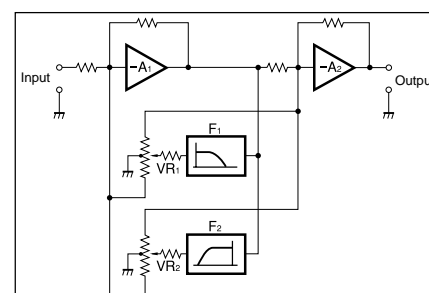
Fig. 6 Tone control circuit diagram (summing active filter type)
