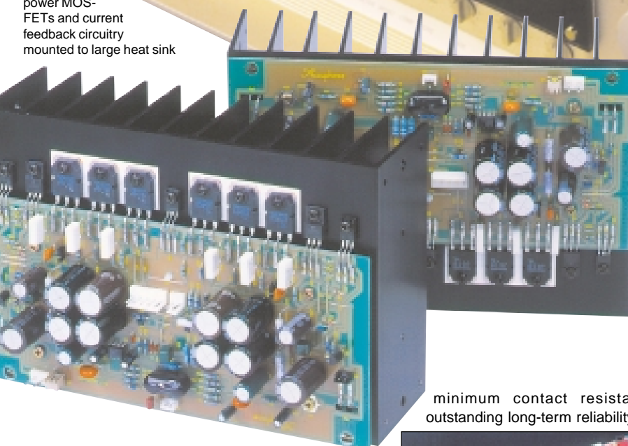
parallel arrangement of input devices helps to minimize noise.
