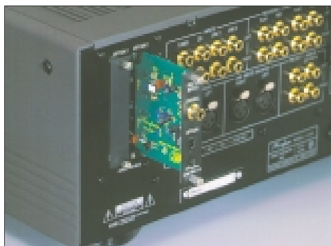
Option board shown in photo is DAC-10
