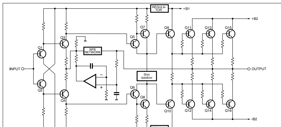
Figure 2 Principle of current feedback amplifier
