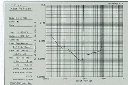
Input voltage vs. total harmonic distortion (input: MC; output: tape output terminal)
