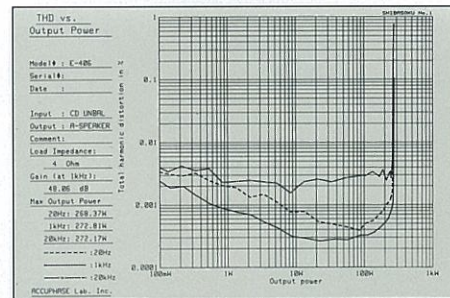
Output power vs. total harmonic distortion (at 4 ohms)
