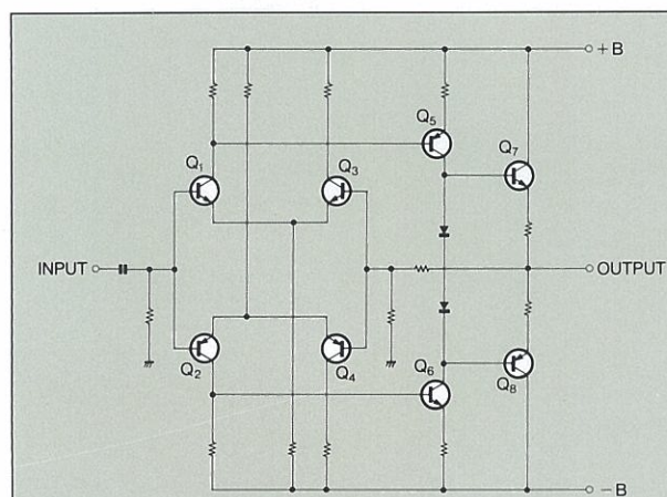
Fig. 2 Circuit Diagram of the Line Amplifier
