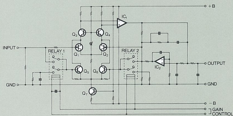
Fig. 3 Circuit Diagram of the Equalizer Amplifier
