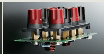
Speaker terminals with thick, short connecting shafts and protection circuitry
