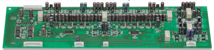
AAVA volume control assembly with increased circuit and parts mounting density
