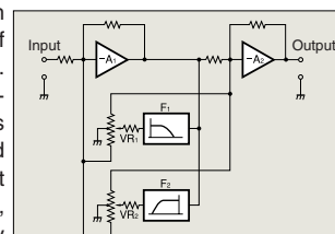
Fig. 5 Tone control circuit principle (Summing active filter type)
