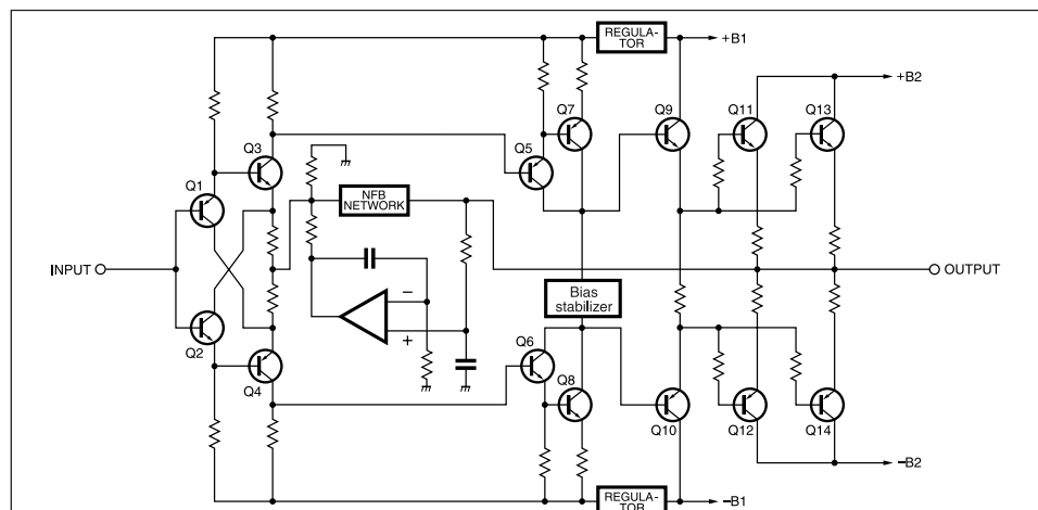
Figure 2 Principle of current feedback amplifier
