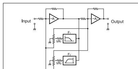
Figure 4 Tone control circuit principle (Summing active filter type)
