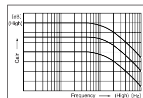
Fig. 3 Frequency response with current feedback (response remains uniform also when gain changes)
