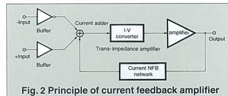
Fig. 2 Principle of current feedback amplifier
