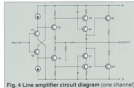
Fig. 4 Line amplifier circuit diagram (one channel)
