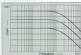
Fig. 3 Frequency response with current feedback (Response does not change when gain is varied)
