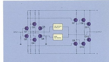
Fig. 3 Circuit Diagram of Head Amplifier
