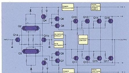
Fig. 1 Circuit Diagram of Power Amplifier
