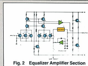
Fig. 2 Equalizer Amplifier Section
