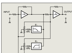
Fig. 5 Tone control circuit principle (Summing active filter type)
