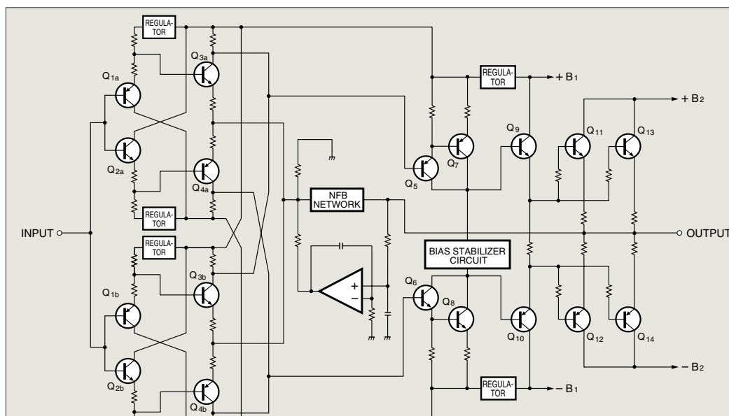
Fig. 2 Circuit diagram of line amplifier (one channel)
