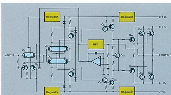
Fig. 1 Power Amplifier Section
