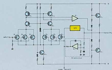
Fig. 2 Equalizer Amplifier Section
