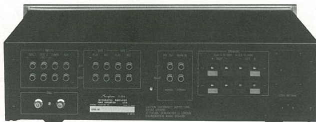
REAR PANEL VIEW
