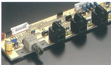
HPC optical and Toslink optical transmitters
