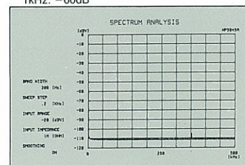
● Spectrum analysis of non-signal reproduced noise vs. frequency characteristic (352.8kHz sampling frequency is attenuated to about 105dB.)
