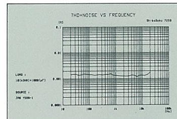
● THD + noise vs. frequency characteristic
