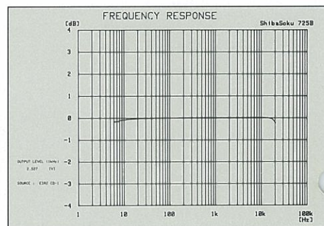
Frequency response
