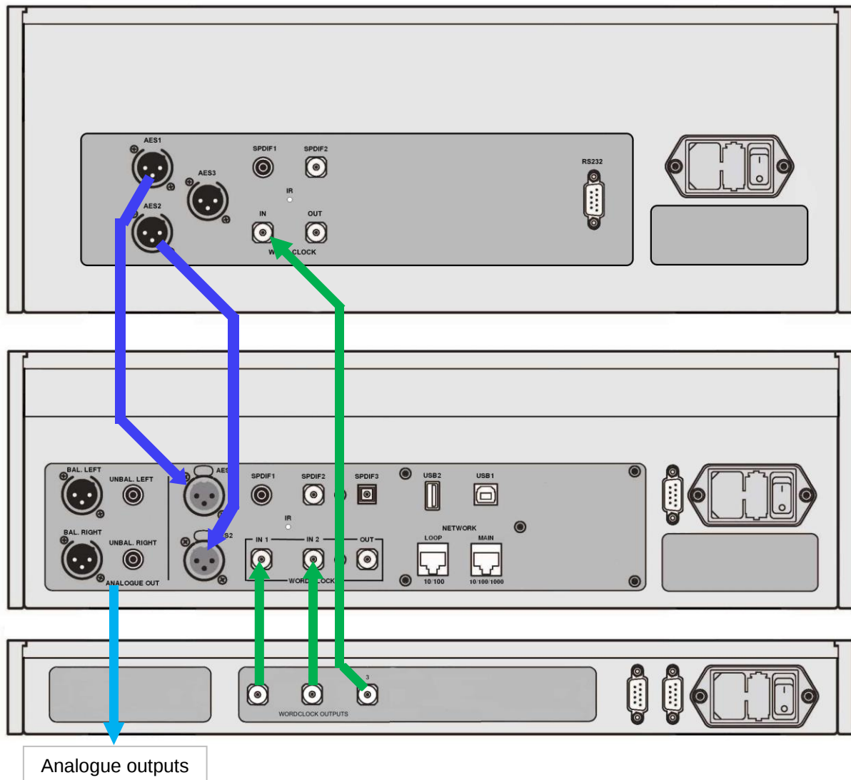
Figure 7 – Using the Rossini Player, Clock and Transport together
