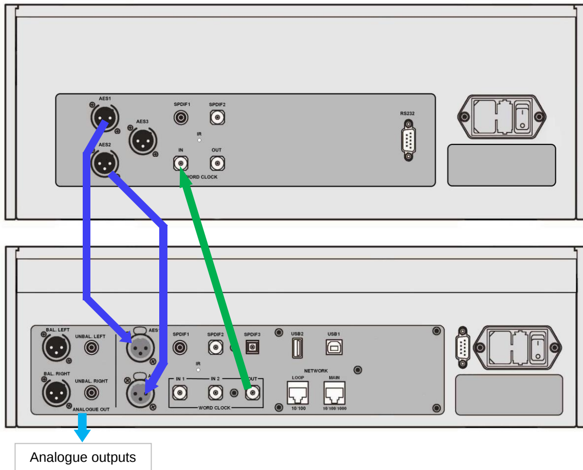
Figure 6 – Using the Rossini Player in Master Mode with a Rossini Transport
