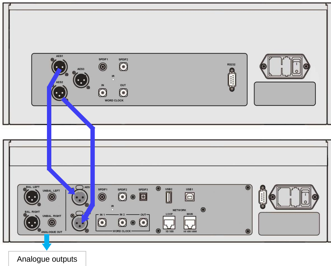
Figure 3 – Using the Rossini Player with the Rossini CD/SACD Transport
