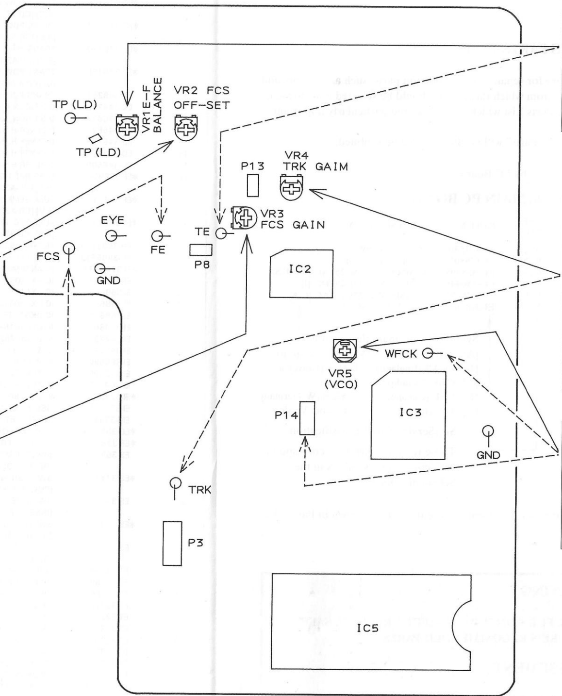
MAIN PCB
