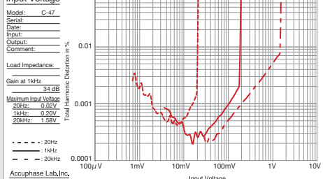
Input voltage vs. THD characteristics (MM input)
