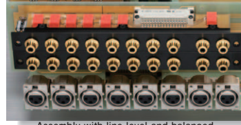
Assembly with line level and balanced input and output connectors
