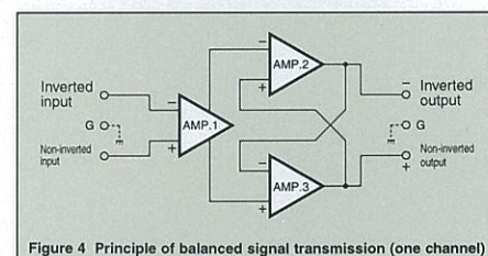
Figure 4 Principle of balanced signal transmission (one channel)
