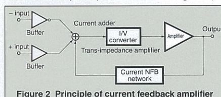
Figure 2 Principle of current feedback amplifier
