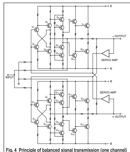
Fig. 4 Principle of balanced signal transmission (one channel)
