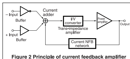
Figure 2 Principle of current feedback amplifier
