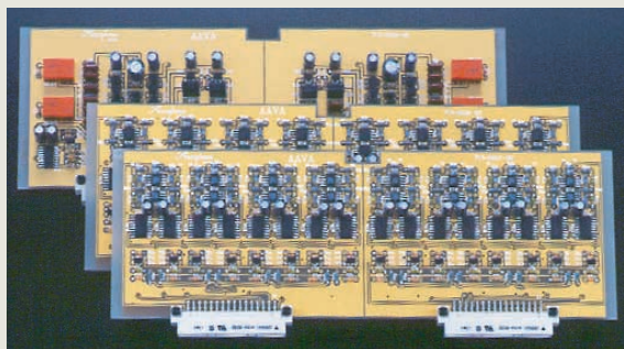
Input buffer, 16 V-I converter amps and current switches, current adder, I-V converter amp, and other circuitry on modular AAVA unit, installed separately for left/right channel on motherboard
