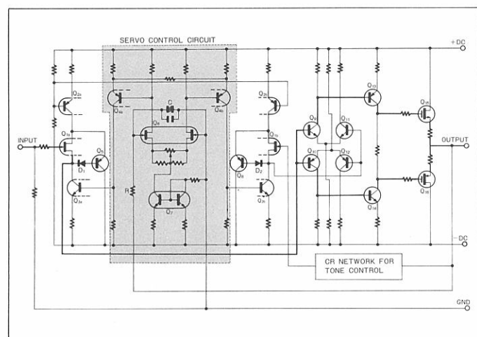
Fig. 1 DIAGRAM OF SERVO CONTROLLED HIGH-LEVEL AMPLIFIER
