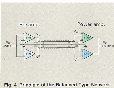
Fig. 4 Principle of the Balanced Type Network
