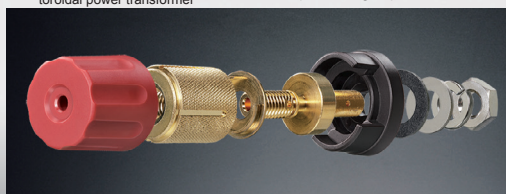
Large gold-plated speaker terminal made of solid brass
