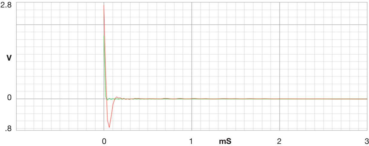
Zu Union-6 Complete Electromechanical Impulse Response Raw (No Filters, No Smoothing)
