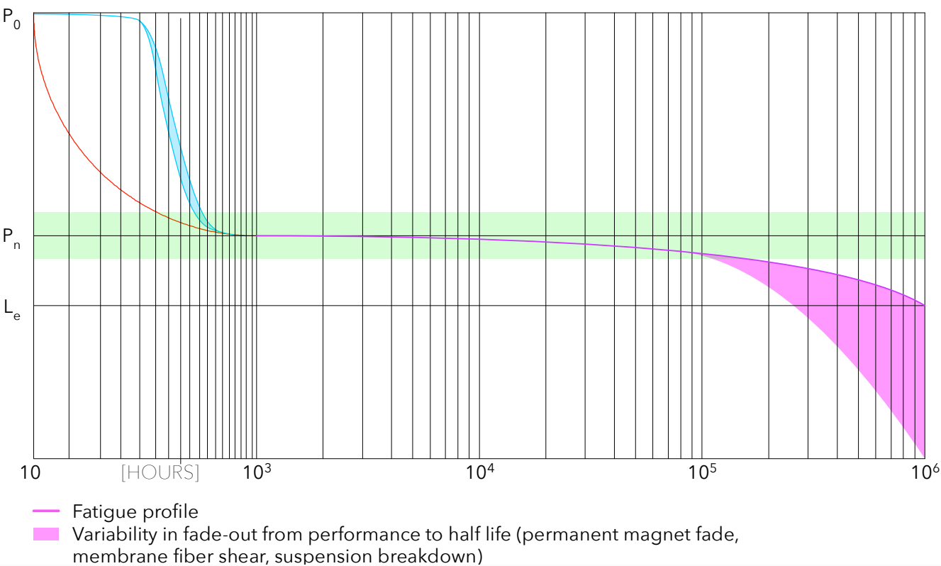
UNION-6 LOUDSPEAKER SYSTEM FATIGUE PROFILE [2/2023]
