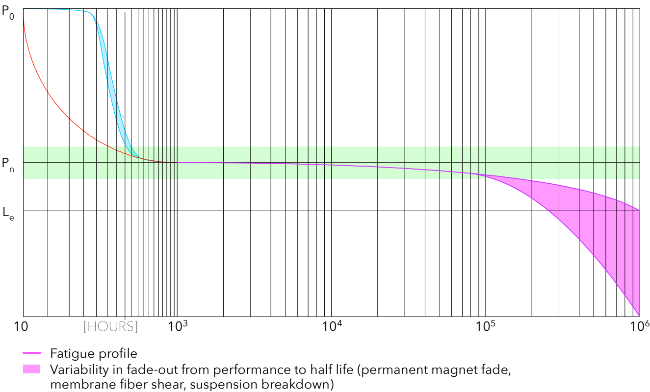
DIRTY WEEKEND-6 LOUDSPEAKER SYSTEM FATIGUE PROFILE [2023]
