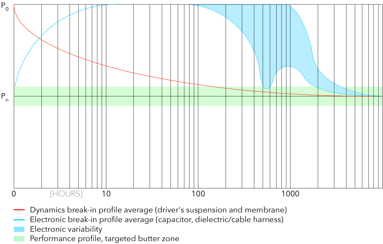
DIRTY WEEKEND-6 SUPREME BURN/BREAK-IN PROFILE [2023]
