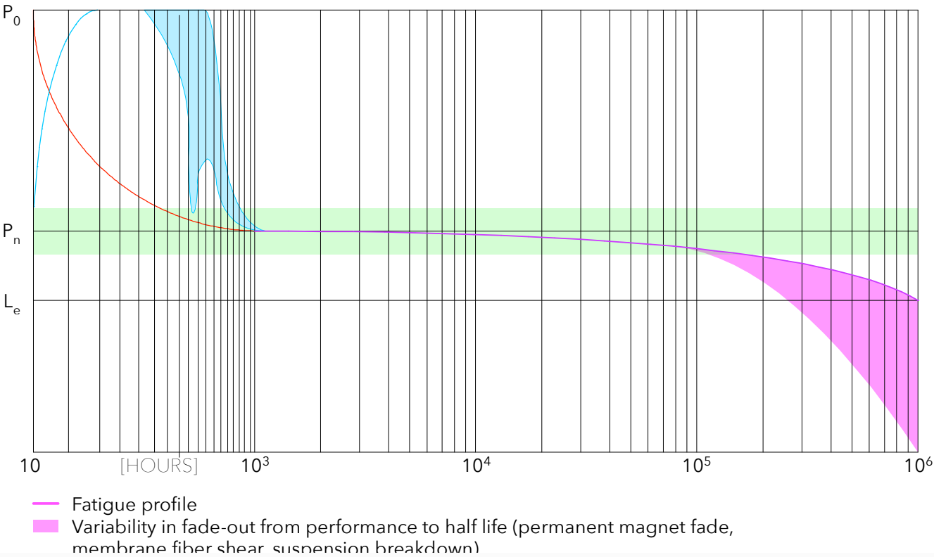
DIRTY WEEKEND-6 SUPREME LOUDSPEAKER SYSTEM FATIGUE PROFILE [2023]
