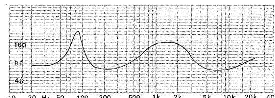
Impedance Characteristic
