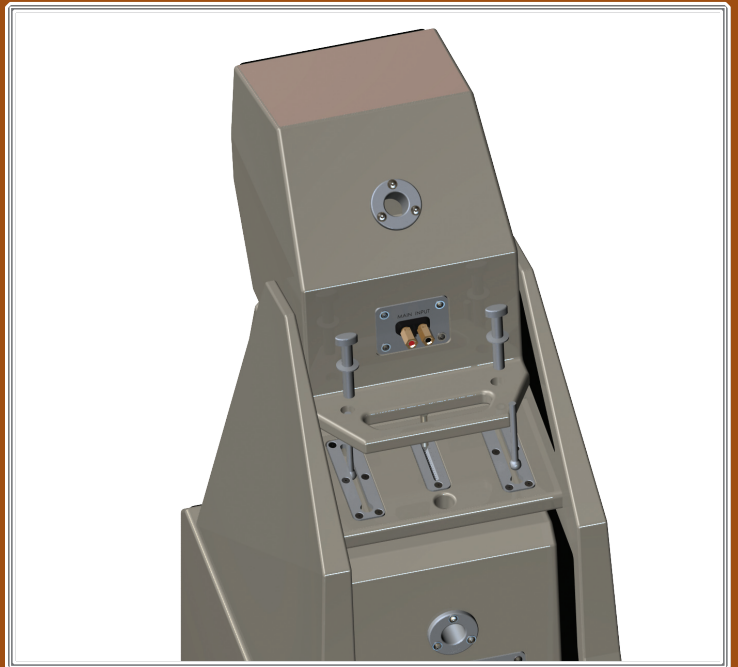
FIGURE 14 - INSTALL THE TETHER BOLTS IN UPPER MODULE
