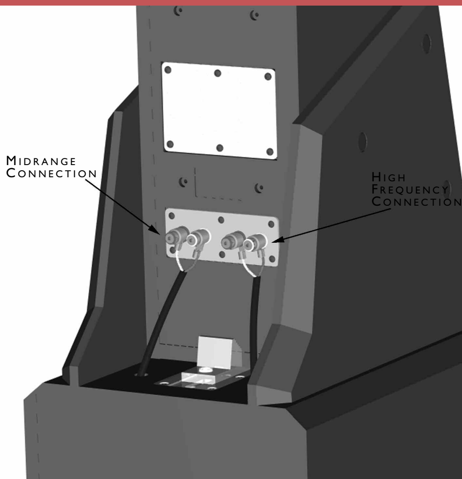
FIGURE 16 - ATTACHING UPPER WIRES
