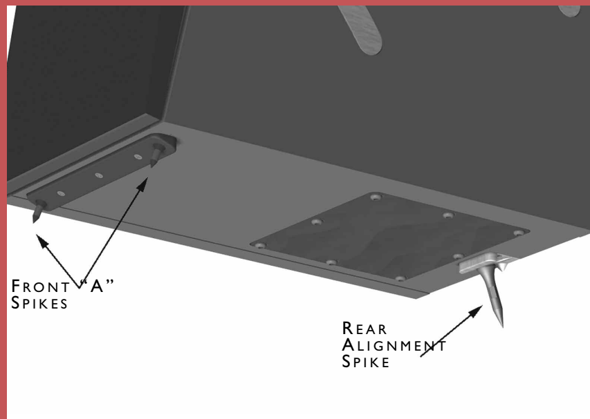
FIGURE 6 - INSTALLING SPIKES INTO THE UPPER MODULE
