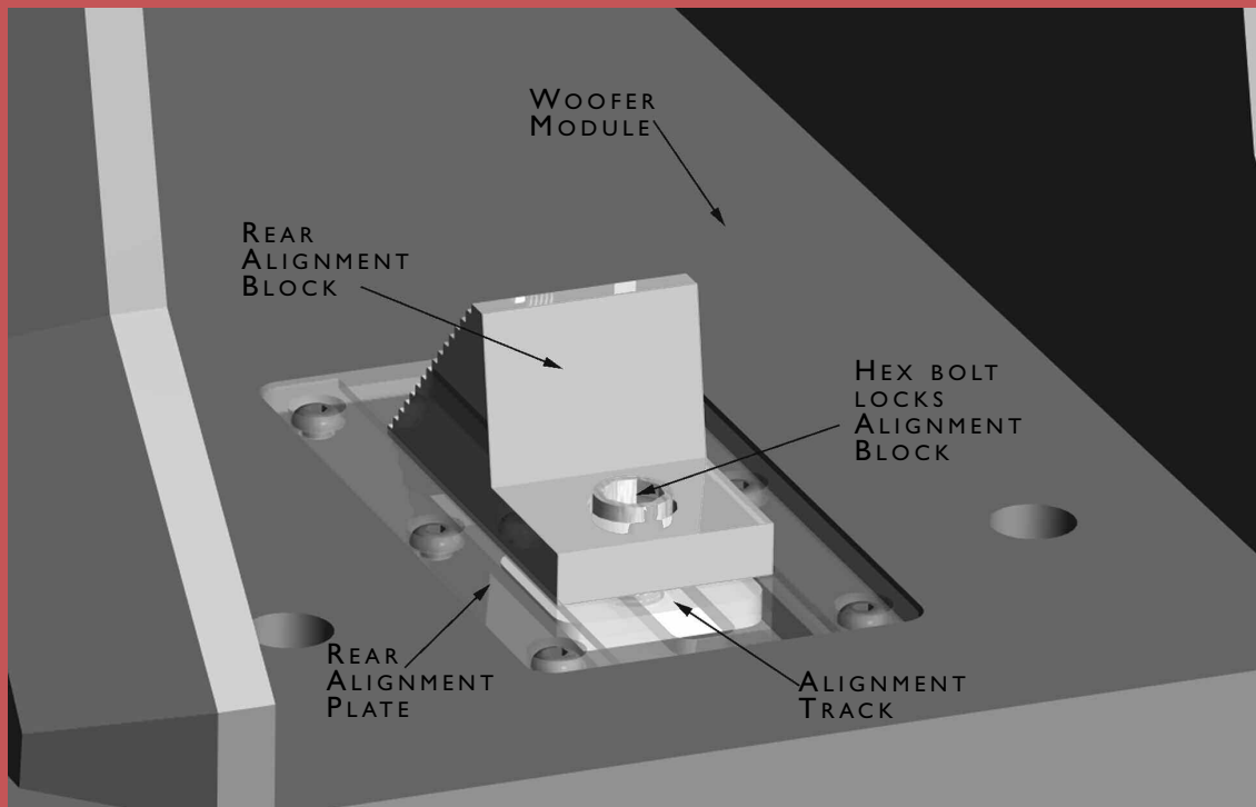
FIGURE 7 - INSTALLATION OF THE ALIGNMENT BLOCK
