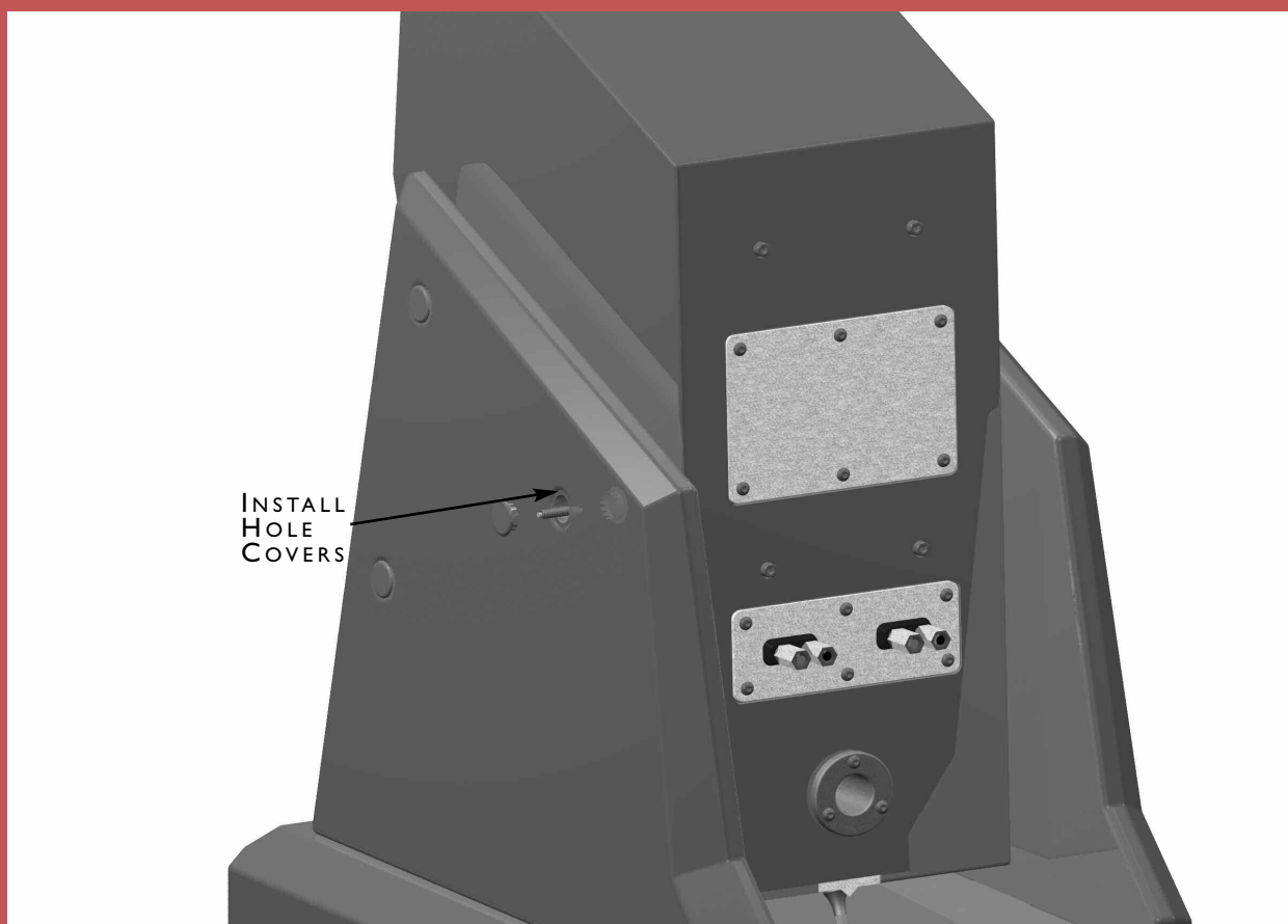
FIGURE 19 - FASCIA HOLES
