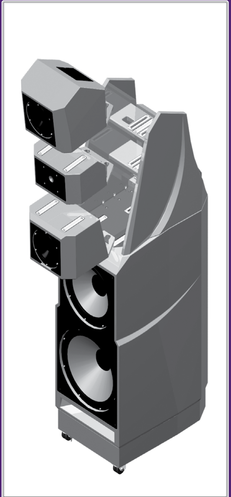
FIGURE 16 - INSTALL THE UPPER MODULES INTO THE WING ARRAY.
