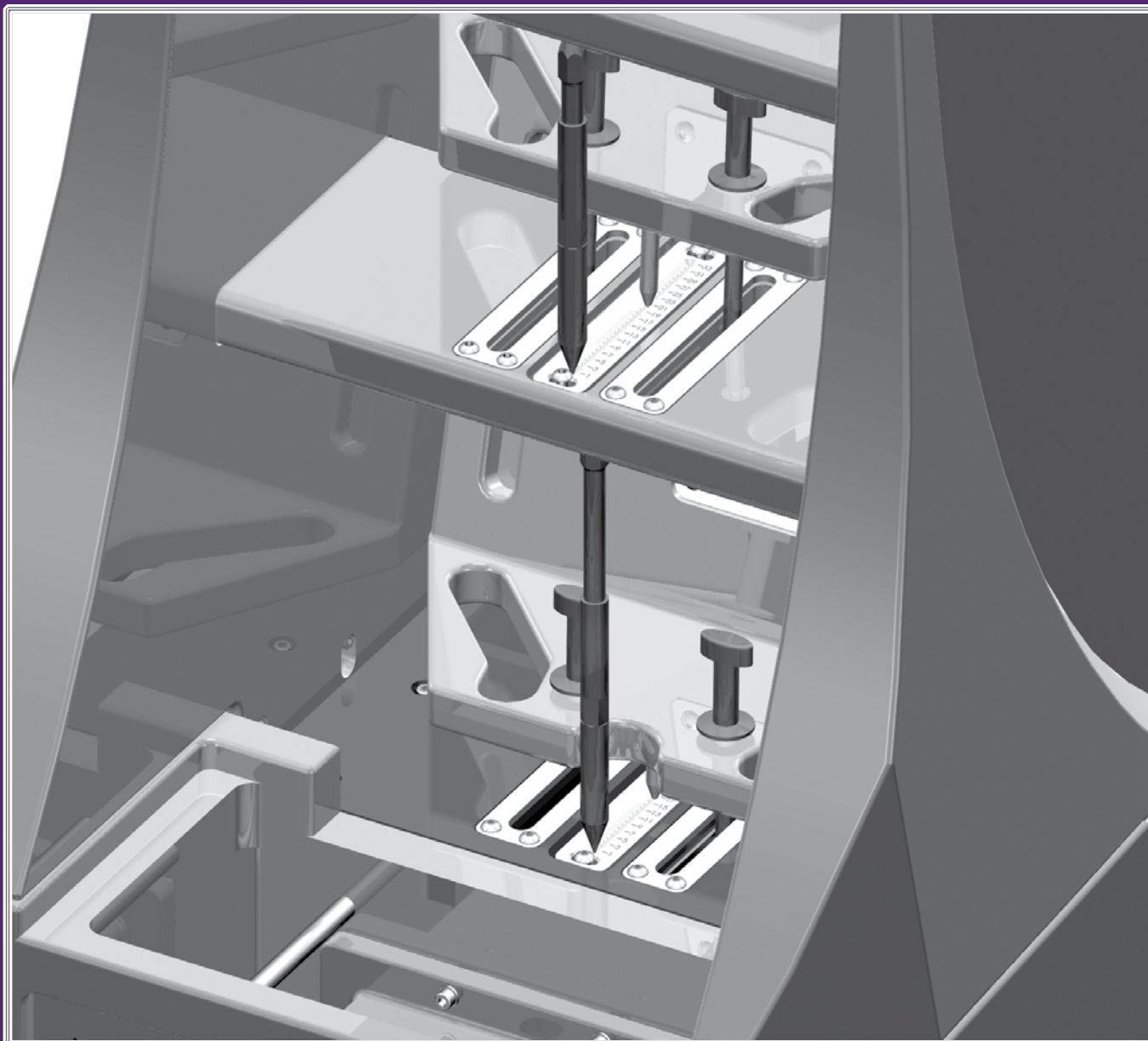
FIGURE 22 - INSTALL THE EXTENSIONS SPIKES.
