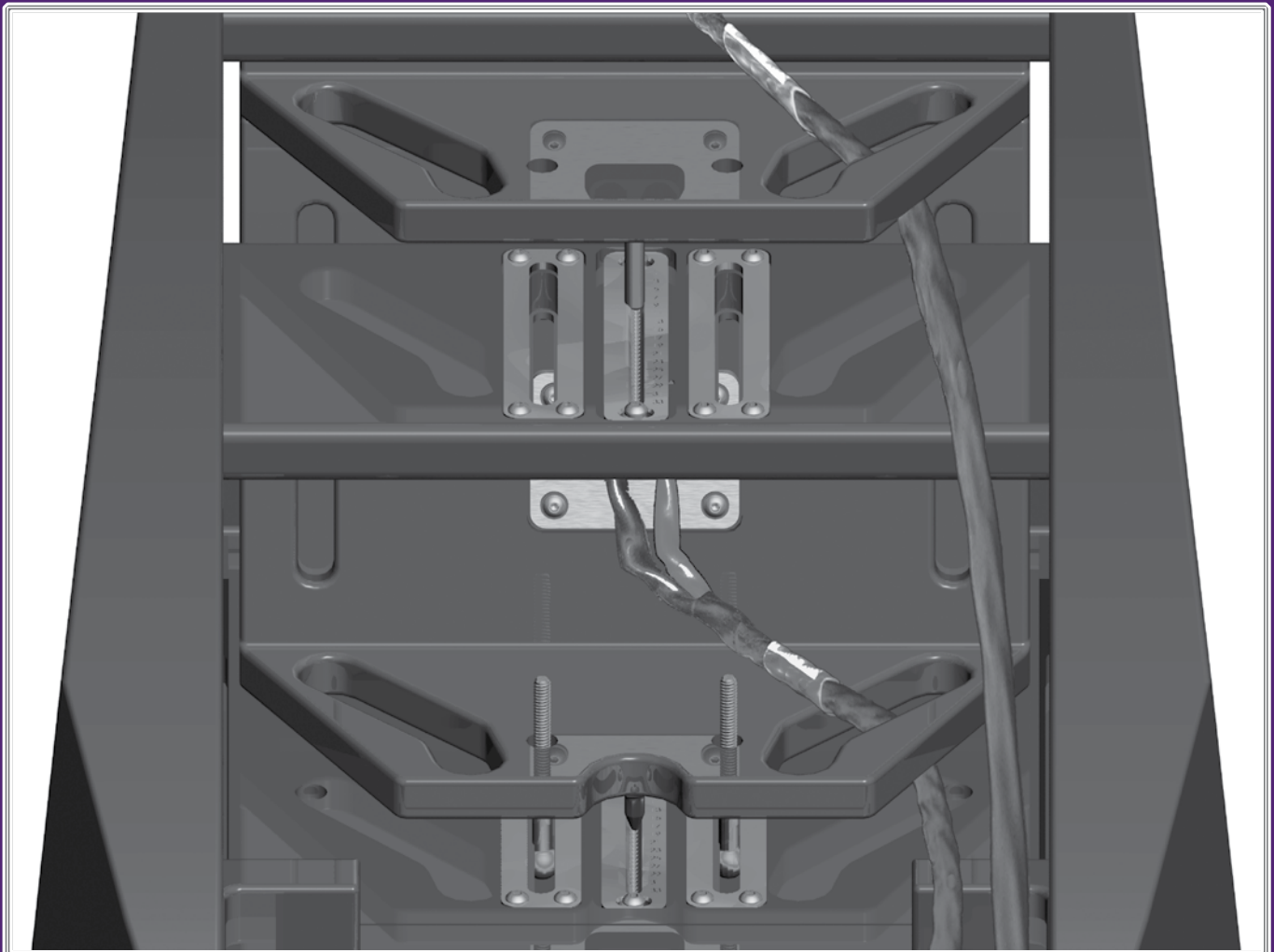
FIGURE 17 - CABLE DRESSING.
