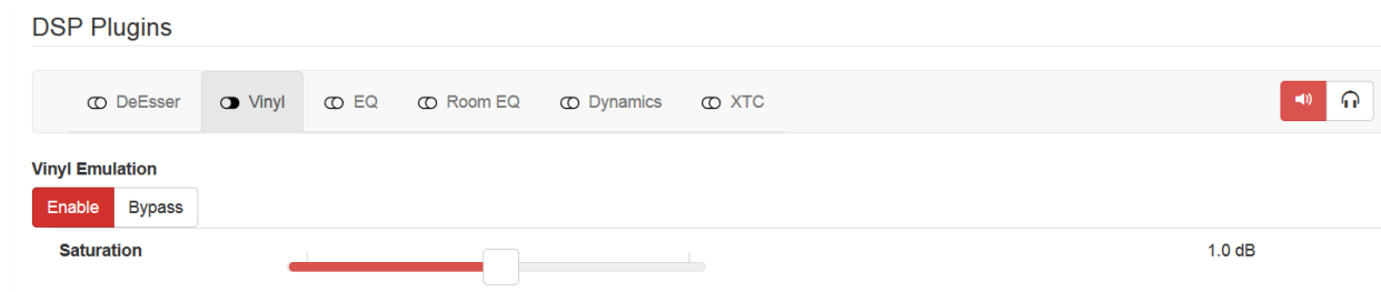
Figure 5: Vinyl plugin
