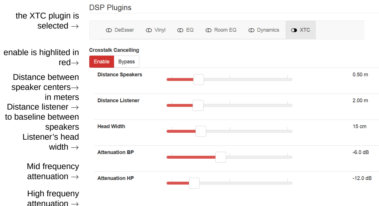
Figure 11: XTC plugin
