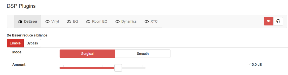
Figure 4: De-Esser plugin
