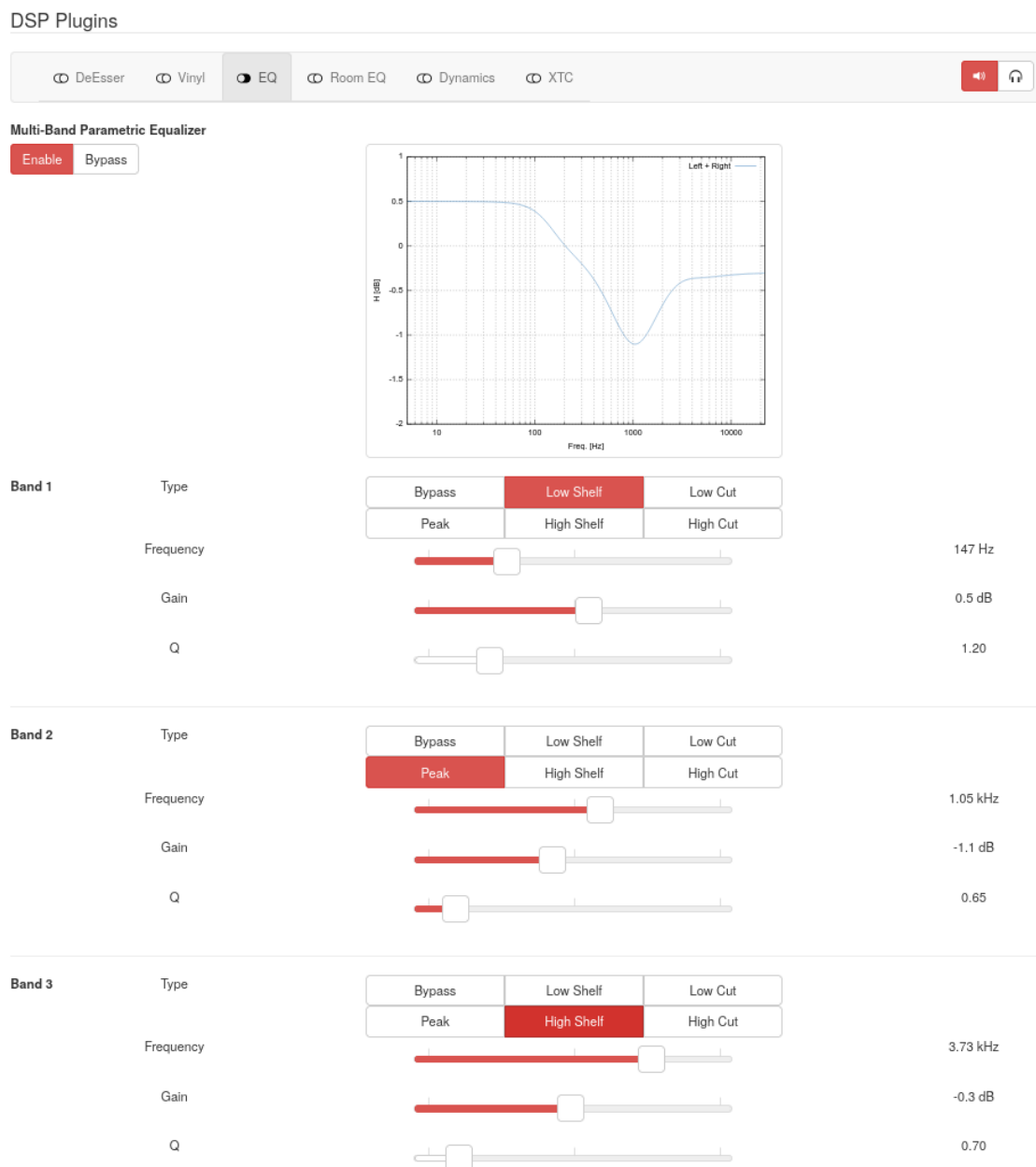
Figure 6: Equalizer plugin
