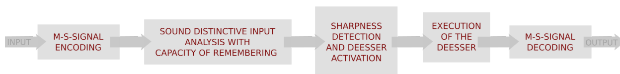
Figure 30: Block diagram of the Weiss De-Esser plugin
