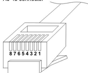
RJ 45 connector
