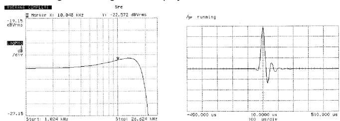
Frequency response and transient characteristics of the Bezier filter
