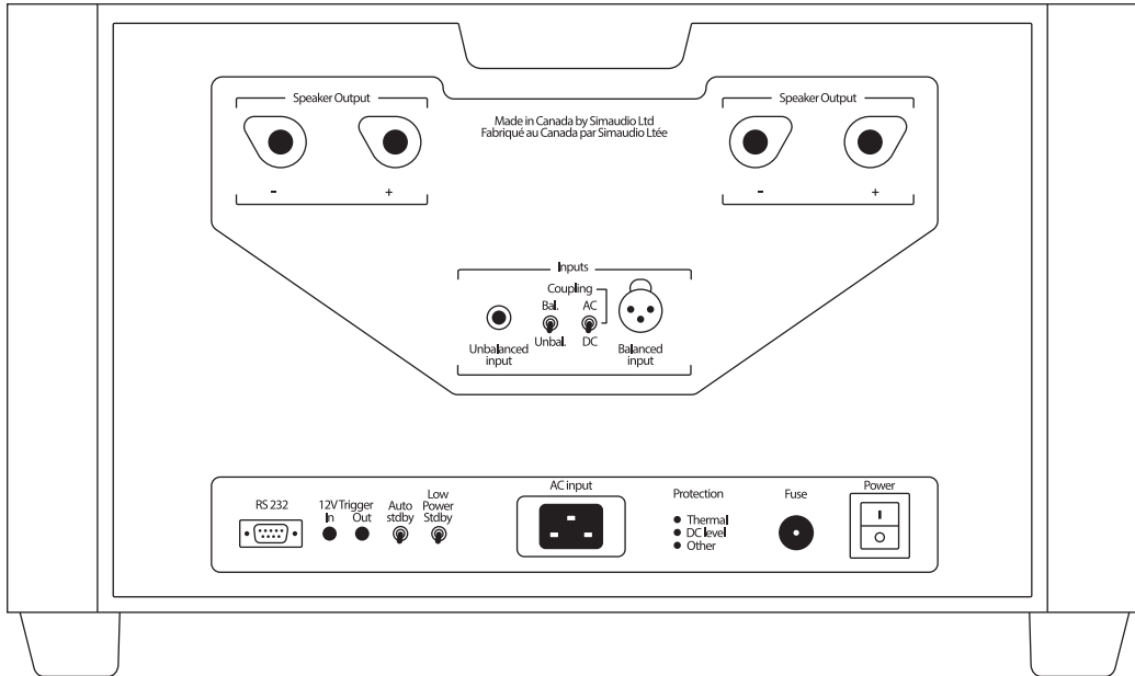
Figure 1: 888 Backpanel
